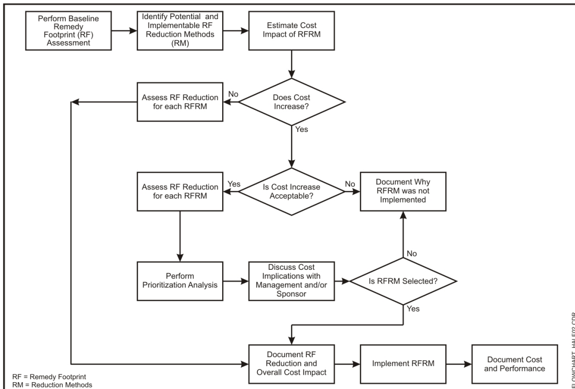
Figure 6-1. Flowchart Representing the General Methodology That Can be Adopted to Reduce the Remedy Footprint During the Design Phase
