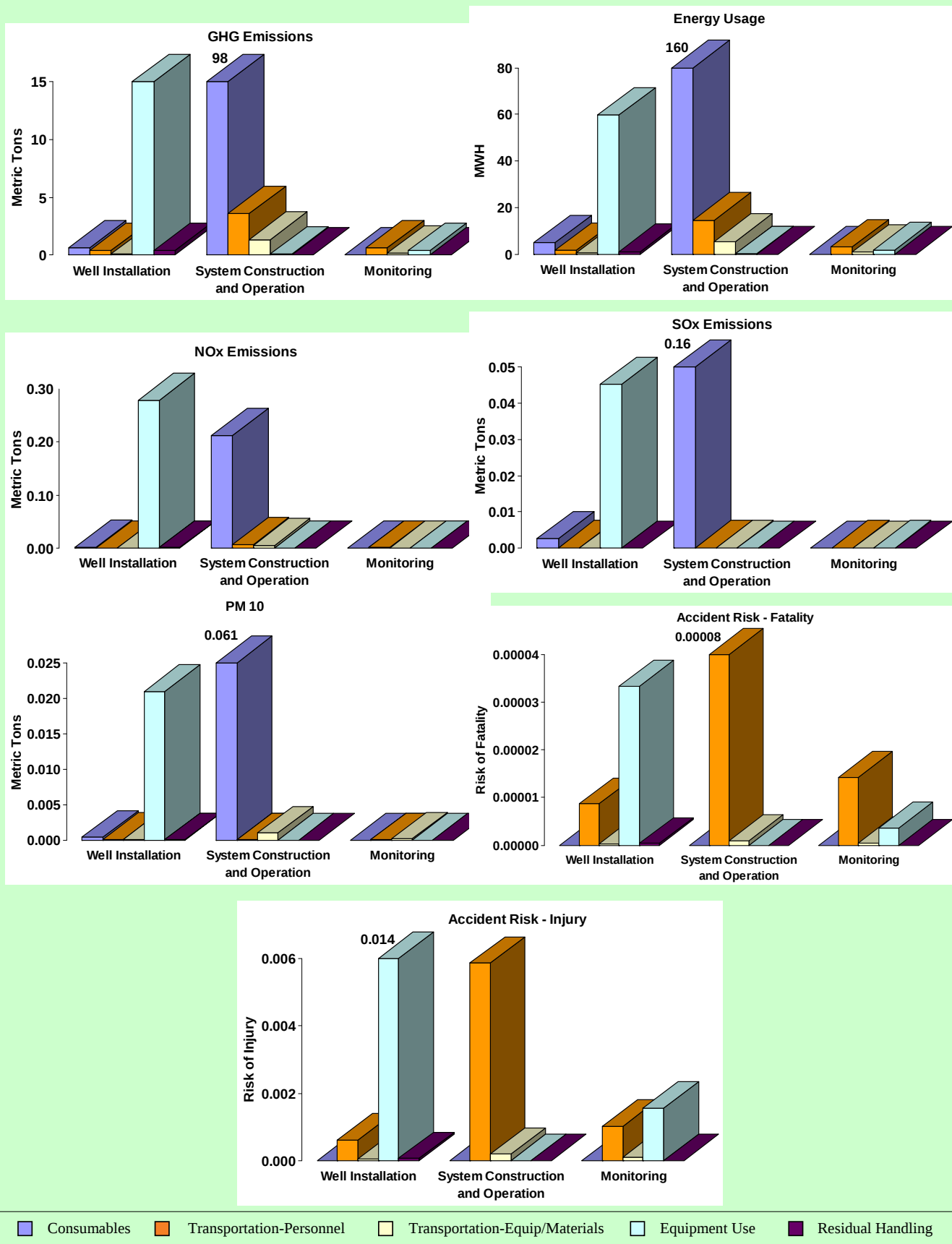
Figure 3. Breakdown of Sustainability Metric Footprint for Shallow Groundwater Alternative ISCO
