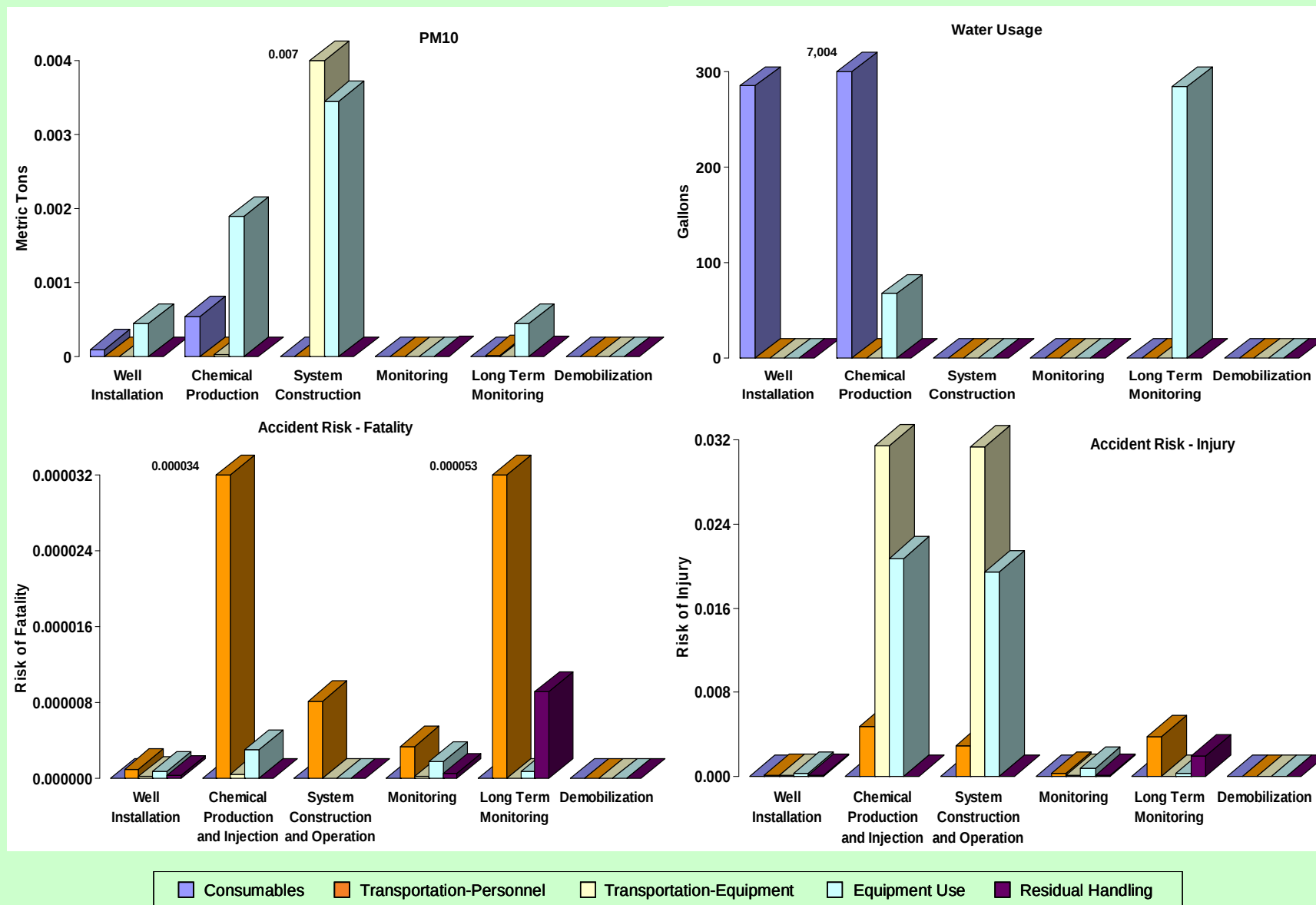
Figure 2. Breakdown of Sustainability Metric Footprint for Remedial Alternative Enhanced Bioremediation (Continued)
