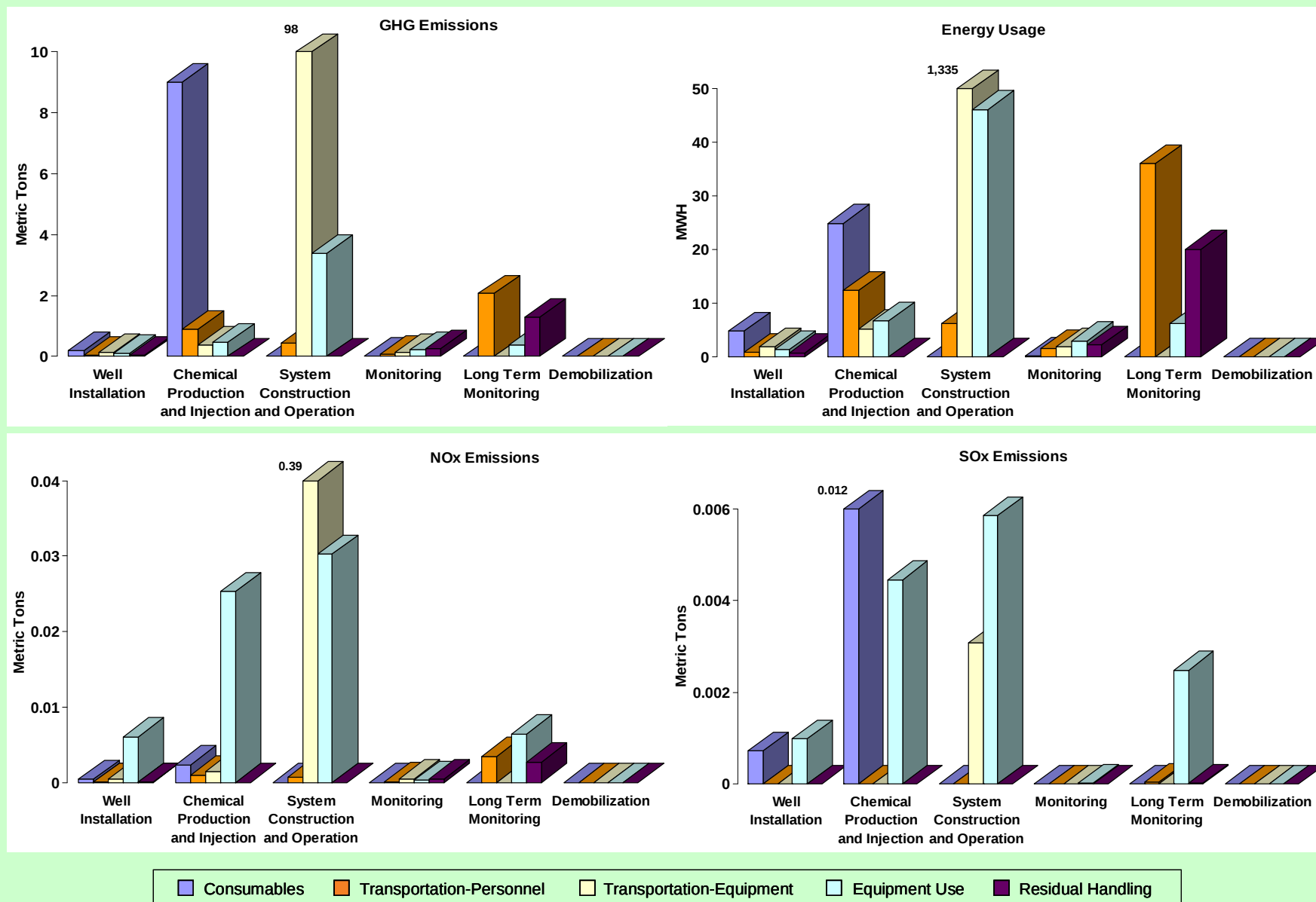
Figure 2. Breakdown of Sustainability Metric Footprint for Remedial Alternative Enhanced Bioremediation
